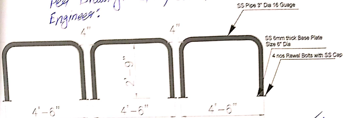
Typical Cafeteria SS Railing Design
